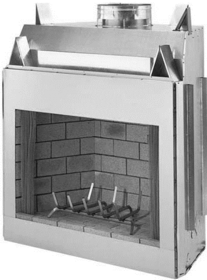
Factory Built ZC Woodburning Fireplace
