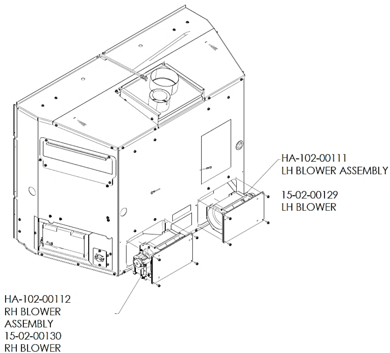
Blower System Parts
