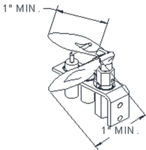
Minimum Pilot Flame Length
